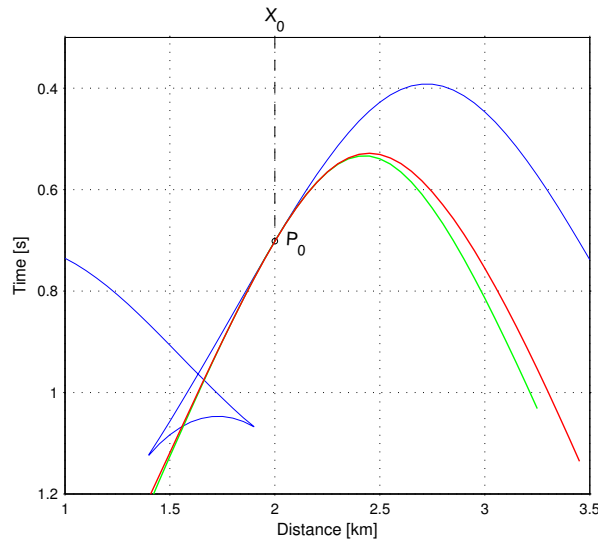
Figure 1: The CDS traveltim curve (green line) and the diffraction traveltim curve (red line) for a normal incidence point on the second reflector. The blue line is the ZO reflection traveltim curve for a second reflector (adapted from Garabito et. al., 2006a).
