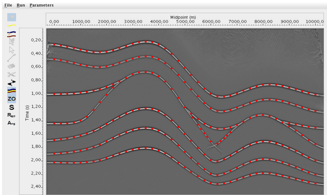
Figure 3: ZO stacked section simulated by CRS stack method. The red points are the picks resulting from semiautomatic picking algorithm.
