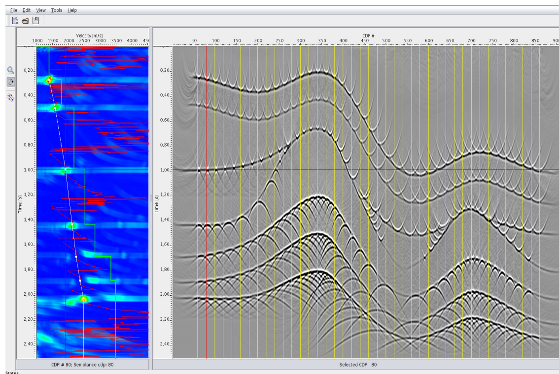
Figure 6: Interactive tool for poststack time velocity analysis by using the velocity spectra (semblance) and the focusing analysis of diffractions.
