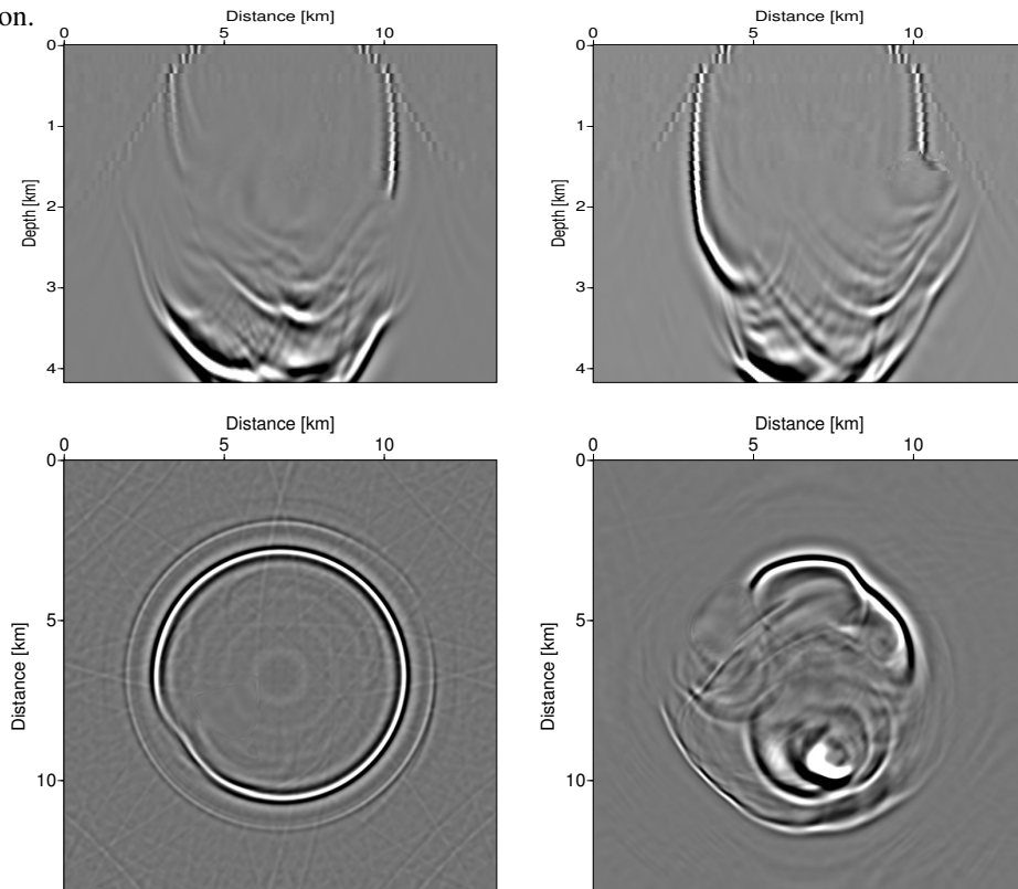
Figure 7: Impulse response obtained by FD migration using complex Padé approximation with 2 terms with rotation angle of 25^\circ and Li correction.
