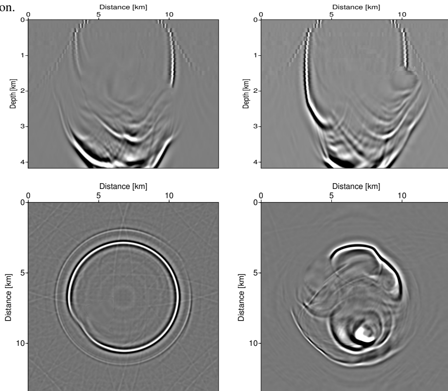
Figure 9: Impulse response obtained by FD migration using complex Padé approximation with 3 terms with rotation angle of 45^\circ and Li correction.
