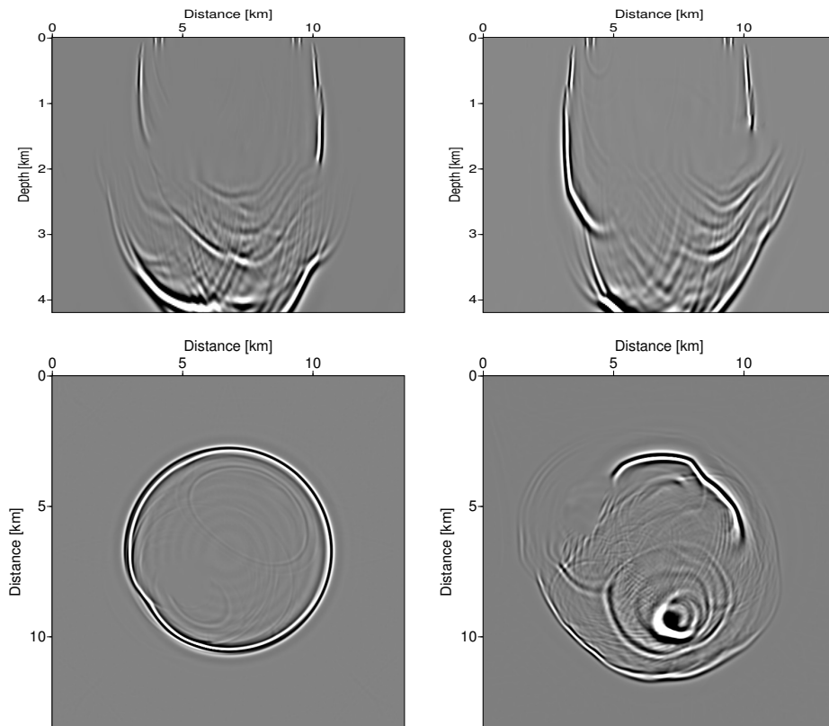
Figure 2: Impulse response obtained by FFDPI migration. 4 cuts represented as x = 8.32 km (top left), y = 8.32 km (top right), z = 1.1 km (bottom left) and z = 2.7 km (bottom right).
