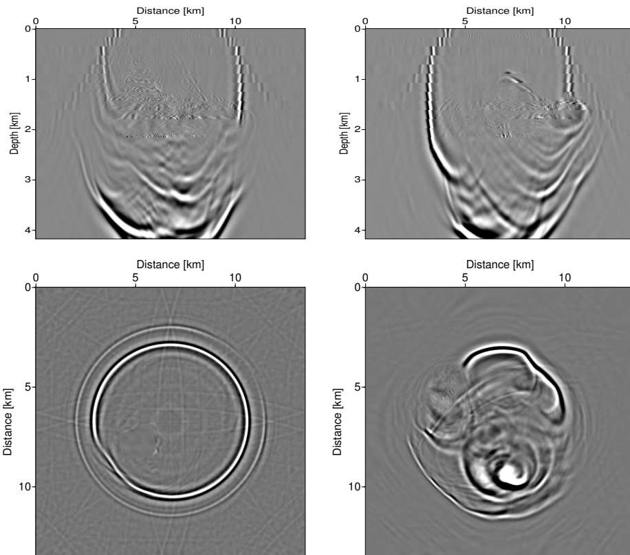
Figure 6: Impulse response obtained by FD migration using real Padé approximation with 2 terms and Li correction.
