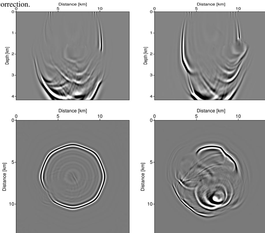
Figure 11: Impulse response obtained by FD migration using alternating four-way splitting and without Li correction.
