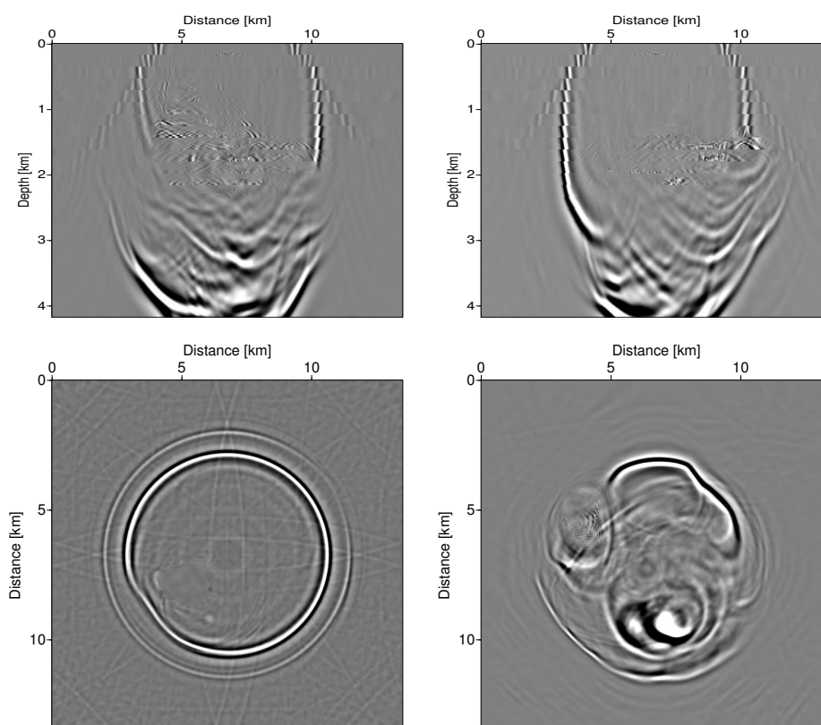
Figure 4: Impulse response obtained by FD migration using real Padé approximation with 1 term and Li correction.
