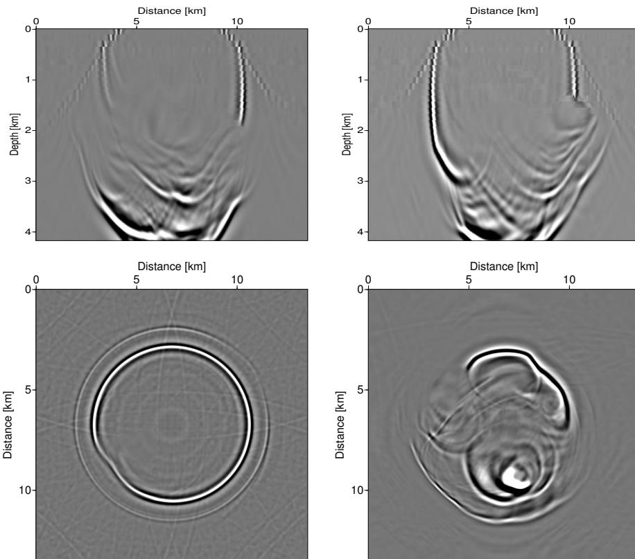
Figure 8: Impulse response obtained by FD migration using real Padé approximation with 3 terms and Li correction.
