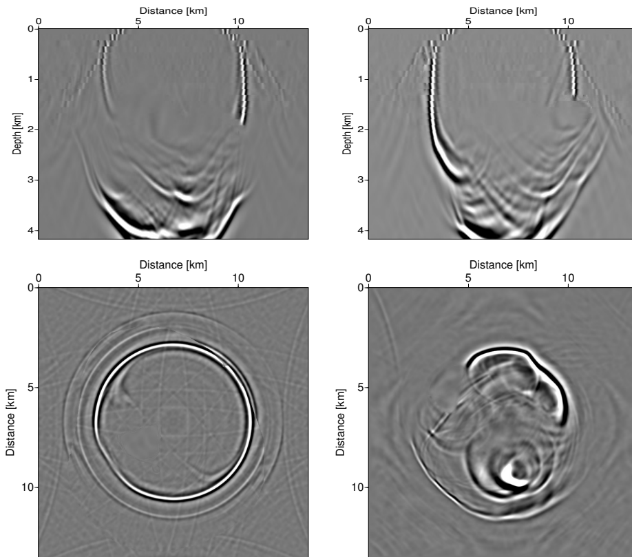
Figure 10: Impulse response obtained by FD migration with rotation angle of 45^\circ , 3 terms, mean slowness, and Li correction.
