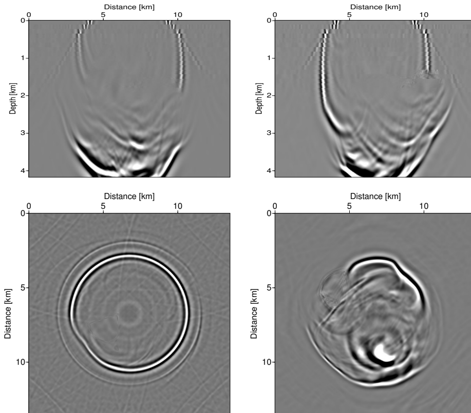
Figure 5: Impulse response obtained by FD migration using complex Padé approximation with 1 term with rotation angle of 15^\circ and Li correction.
