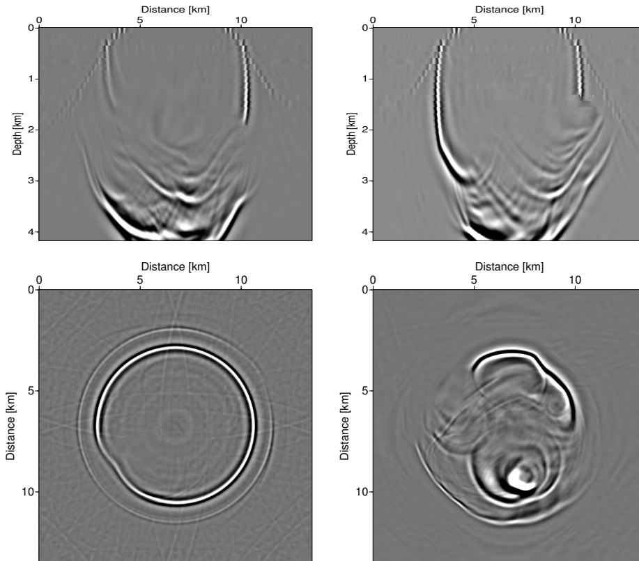
Figure 12: Impulse response obtained by FD migration using alternating four-way splitting and with Li correction.
