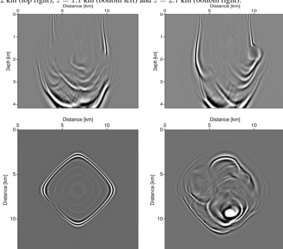
Figure 3: Impulse response obtained by FD migration without Li correction and complex Padé approximation.
